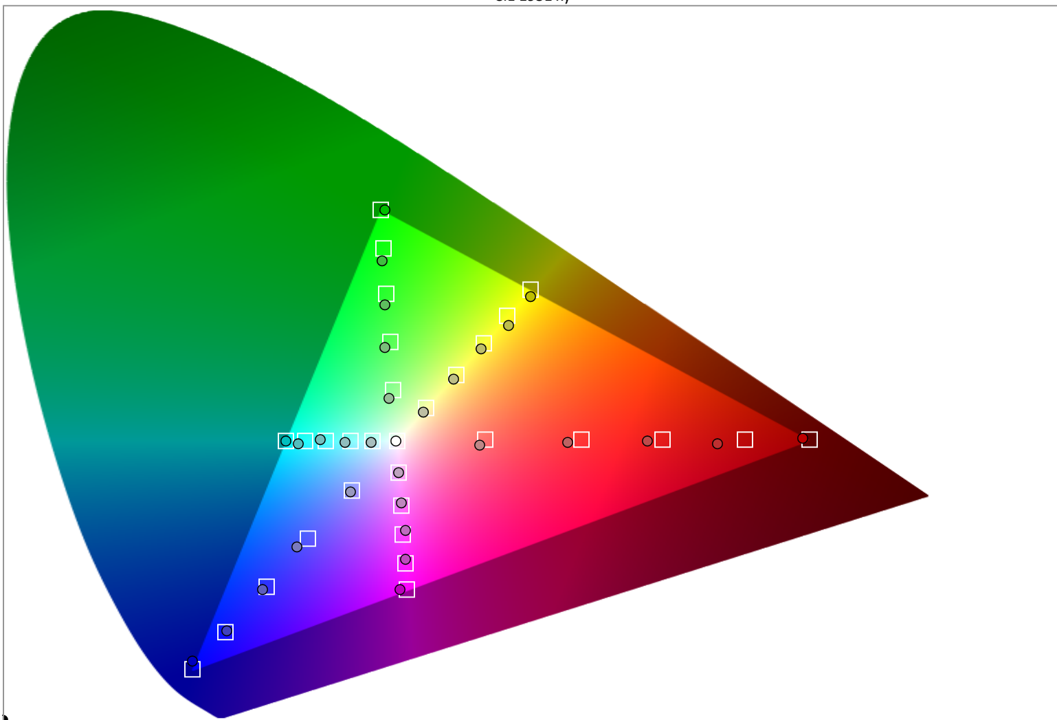
CIE 1931 xy
