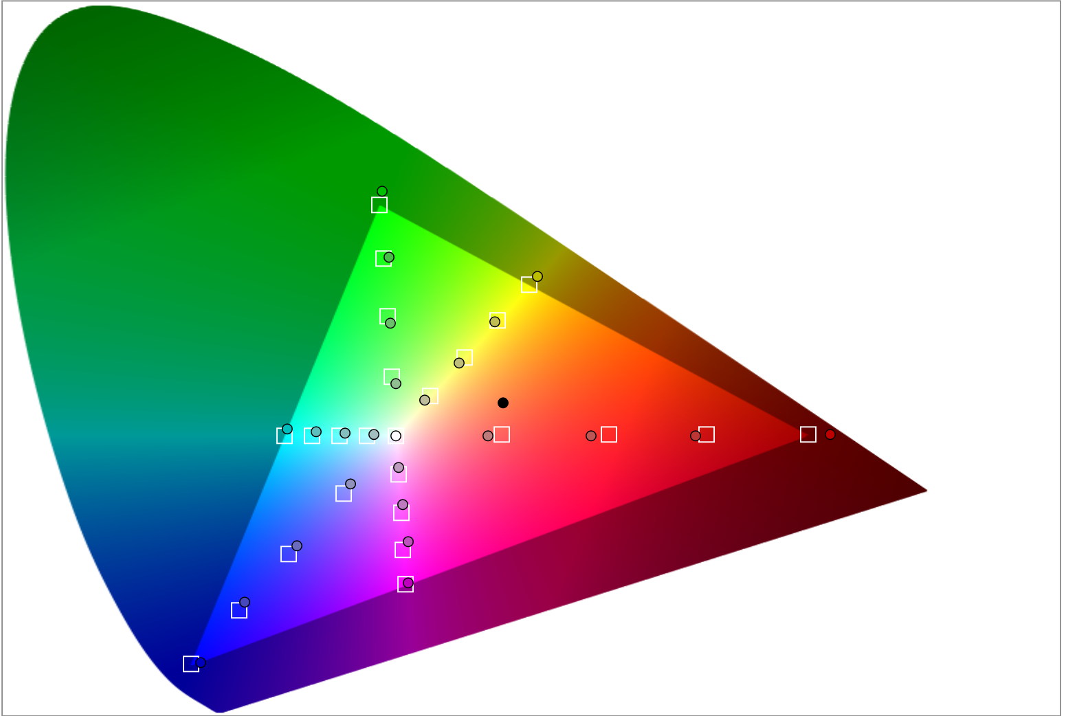
CIE 1931 xy
